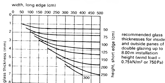
④ Recommended thicknesses, 8m high glass
